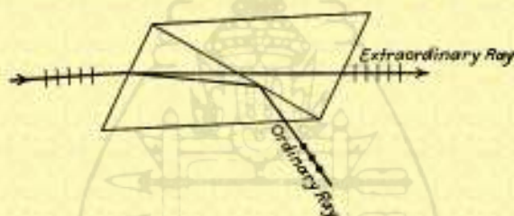
FIG. 49.—The Nicol prism, showing deflection of the ordinary ray.
