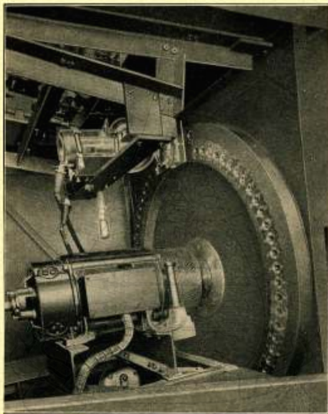
FIG. 56.—The optical system which projects the concentrated illumination output of the neon-glow tube to the eye. A large collecting lens gathers most of the light flux which is projected to the eye through the lenses of the scanning disc.
