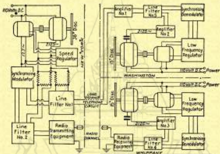
FIG. 64.—Schematic diagram of synchronizing circuits used in the Bell System Washington-New York 50-line radio and wire television demonstration.
