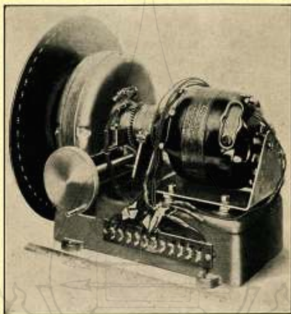
FIG. 65.—The 2,125-cycle synchronous motor, with 120 pairs of poles, used to drive the reproducing scanning disc. The worm drive is used to adjust framing.
