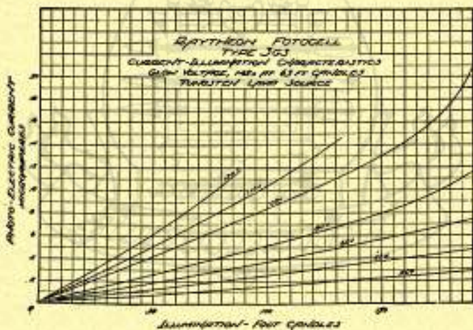
Fig. 26.—Characteristics of Raytheon 3G3 photoelectric cell.
