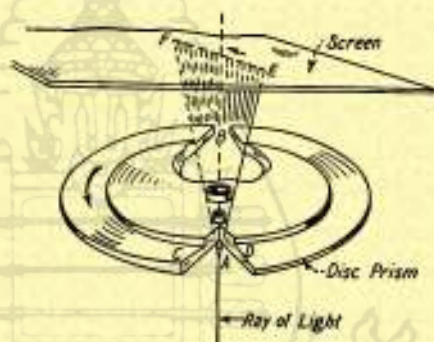
FIG. 18.—As the prismatic disk revolves, the image oscillates along path EF.
