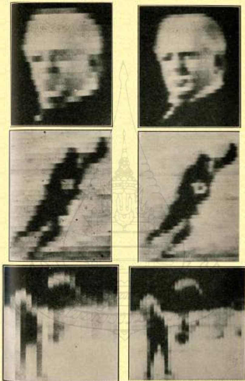
FIG. 66—The three pictures on the left are representative of the definition attainable if the picture signal is confined to a single broadcast channel; those at the right consist of 1,250 picture elements, which can be transmitted through 40,971, the equivalent of two broadcast channels. (Courtesy of Bell Telephone Laboratories.)
