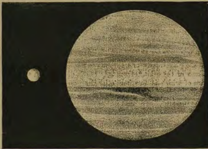
Fig. 88.—Comparative dimensions of Jupiter and the Earth.
