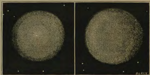
Fig. 117.—1. Tailless Comet. 2. Head without tail or nucleus.
