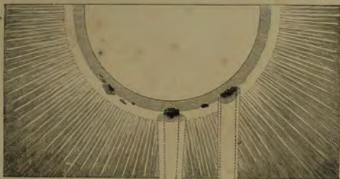
Fig. 18.—Explanation of Sun-spots on Kirchhoff's hypothesis.
