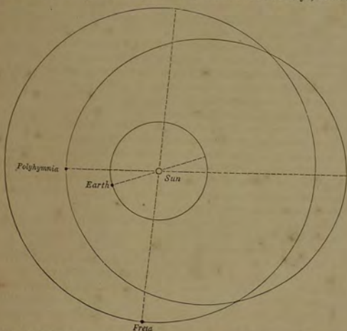
Fig. 53.—Orbits of Freia and Polyhymnia, compared together, and with that of the Earth.
