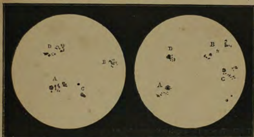
Fig. 11.—Transformation of groups of Solar spots in the interval of a rotation. Observed by M. Pastorf on 24th May and 21st June, 1828.
