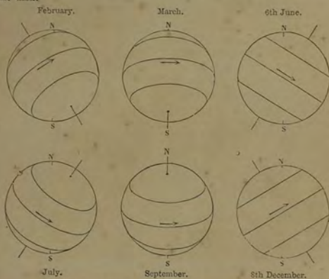
Fig. 8.—Different paths of Sun-spots at different periods of the year.
