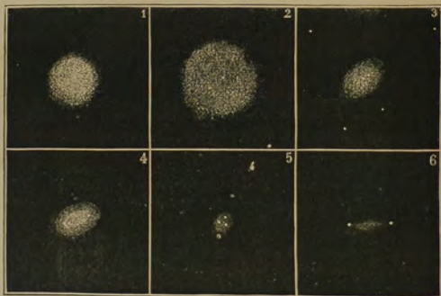
Fig. 168.—Nebulous stars. (Sir J. Herschel.)
