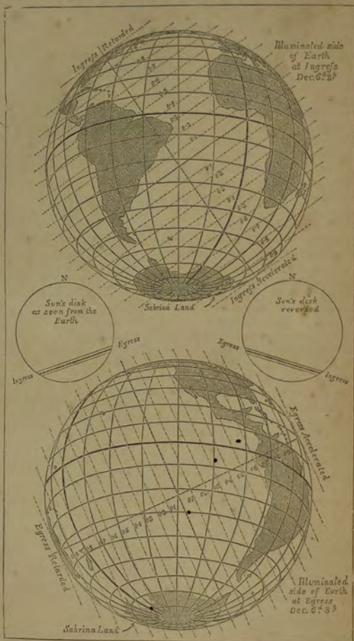
Fig. 184.—Transit of Venus, 1882.
