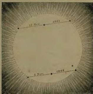
Fig. 27.—Transits of Mercury over the Sun, 1 st the 12 th November, 1861, 2 d the 5 th November, 1868.
