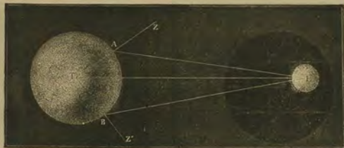
Fig. 182.—Measure of the distance of the Moon.
