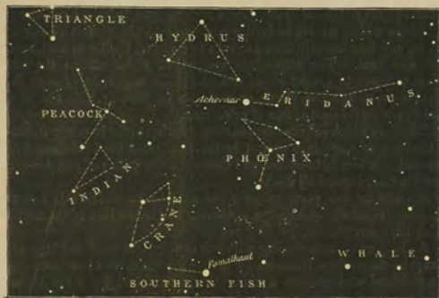
Fig. 137.—Stars invisible at London. Southern Circumpolar zone.
