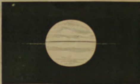
Fig. 101.—Saturn, Nov. 22, 1848 (Bond). Luminosa points visible near the period of the disappearance of the ring.
