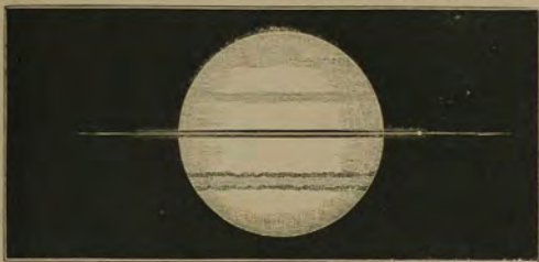
Fig. 99.—Saturn, Jan. 5, 1862, at 14^{\circ} 0' . Luminous appendages of the ring. (Wray.)
