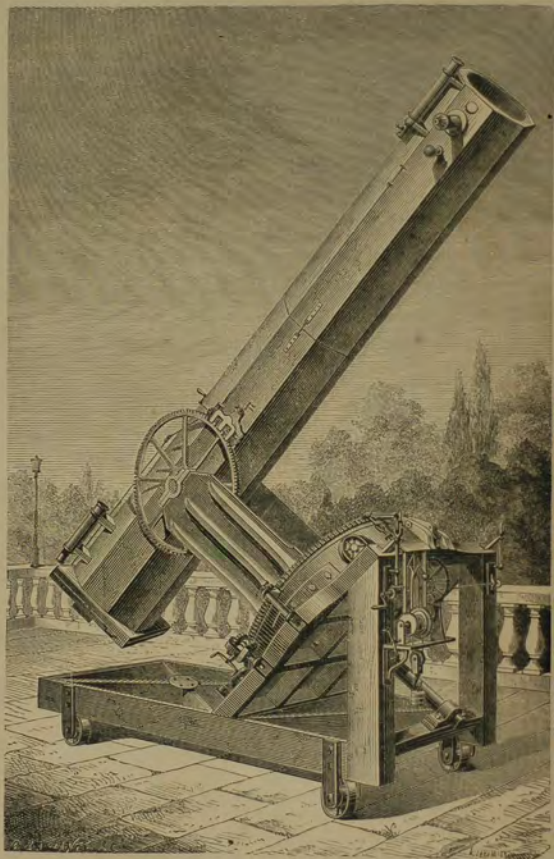
GREAT SILVER-ON-GLASS REFLECTOR. Constructed by M. Foucault.
