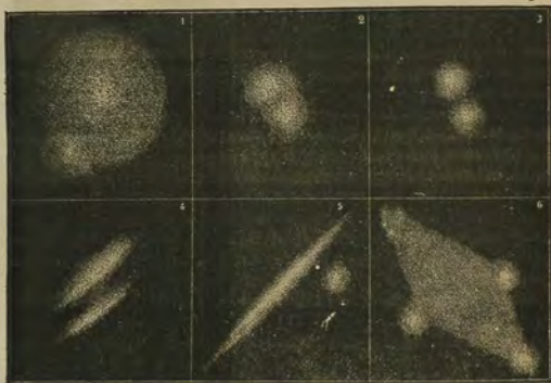
Fig. 170.—Double and multiple nebulae (Sir J. Herschel.)—1 and 4. In Virgo. 2 and 5. In Coma Berenices. 3. In Aquarius. 6. In the Nubecula Major (Great Cloud of Magellan).
