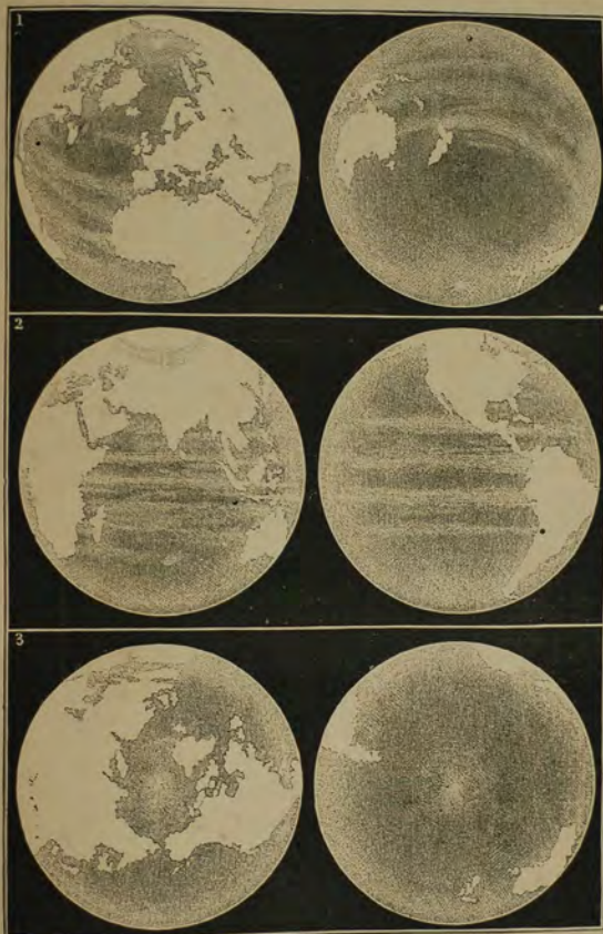
THE EARTH VIEWED FROM SPACE.
