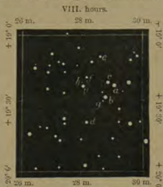
Fig. 140a.—Variable Star Chart. U Cancri. (Knott.)
