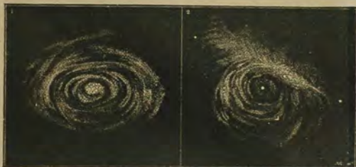
Fig. 158.—Spiral nebulae. (Lord Rosse.)—1. Of the Lion. 2. Of Pegasus.
