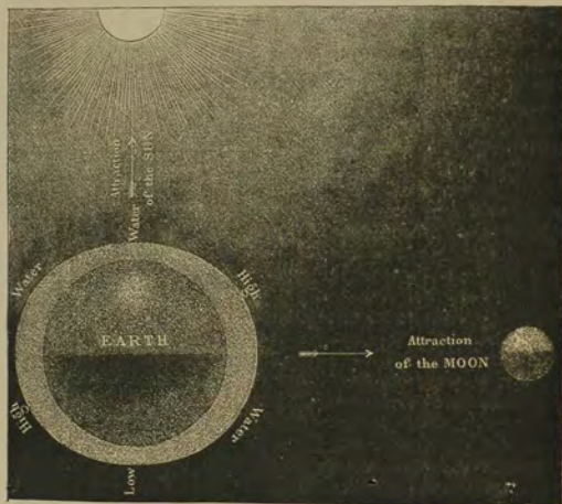
Fig. 180.—Neutralising action of the Moon and Sun on the waters of the sea. Luni-solar tides of the quadratures.
