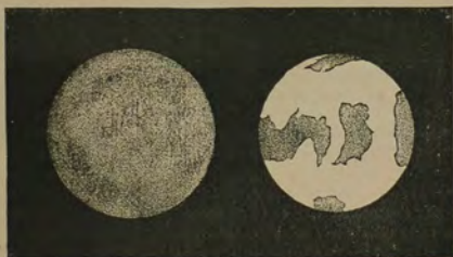
Fig. 34.—Comparative dimensions of Venus and the Earth.
