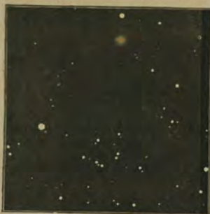
Fig. 145.—The Hyades. (Harding.)
