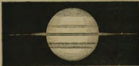
Fig. 98.—Saturn, Dec. 26, 1861, at 15^{\circ} 26' . (Wray.) Luminous appendages of the ring. The satellites are also seen apparently on the ring.
