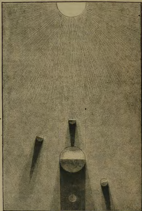
Fig. 65.—General theory of Eclipses
