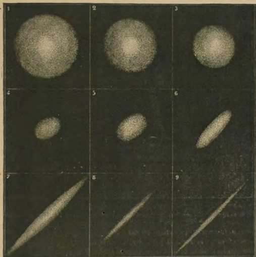
Fig. 151.—Nebulæ of circular and oval forms. (Sir J. Herschel.)
