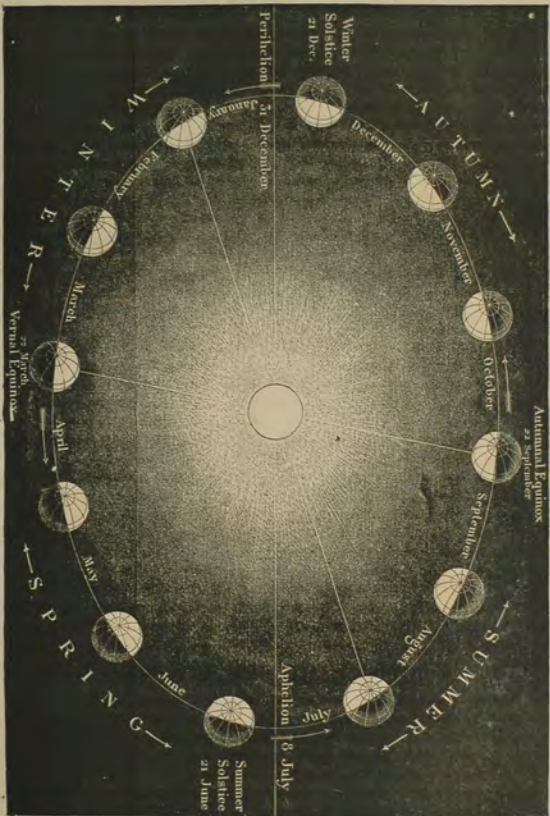
ORBIT OF THE EARTH.
