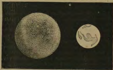
Fig. 79.—Mars and the Earth; comparative dimensions.
