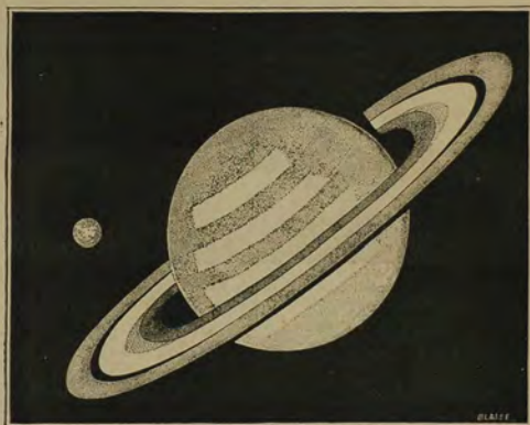
Fig. 96.—Saturn and the Earth; Comparative dimensions.
