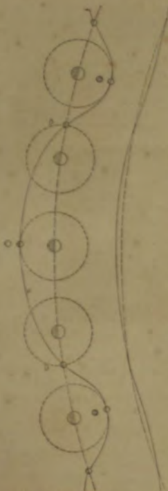
Fig. 37.—The lunar Orbit. 1. Amplified. 2. In its relative dimensions.
