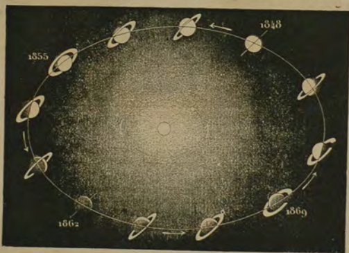
Fig. 100.—Explanation of the Phases of Saturn's rings. Periodical disappearances of the rings.
