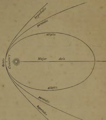
Fig. 119.—Form of cometary orbits.
