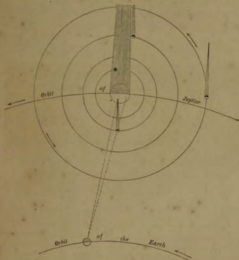
Fig. 53.—Eclipses and passages of the Satellites of Jupiter, seen from the Earth.
