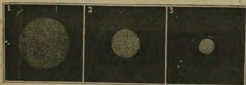
Fig. 166.—Planetary nebula. (Sir J. Herschel.) 1. In Ursa Major. 2. In Pisces. 3. In Andromeda.
