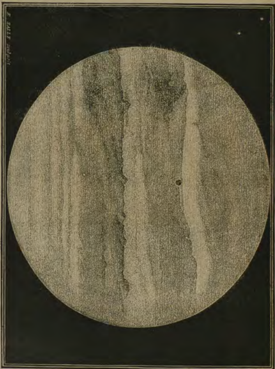
Bright and dark belts, transit of a Satellite and its shadow across the disk. (Warren De La Rue.)
