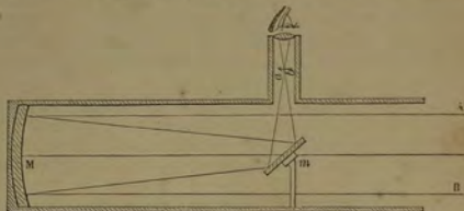
Fig. 188.—Newtonian Reflector.
