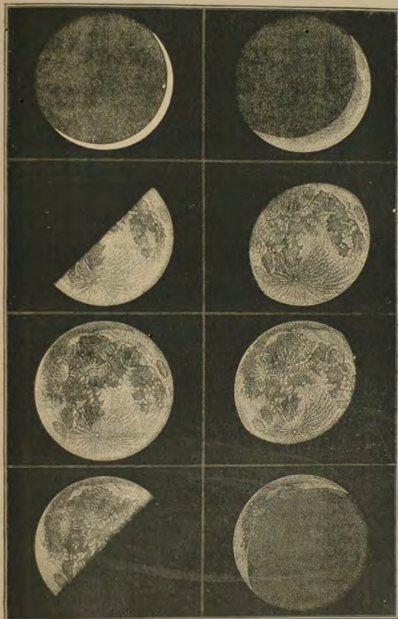
THE PHASES OF THE MOON.
