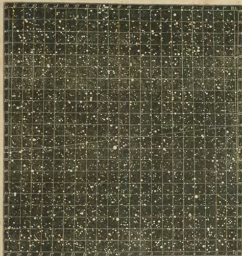
Fig. 55.—Ecliptic chart, from M. Chacornac's 'Star Atlas.'
