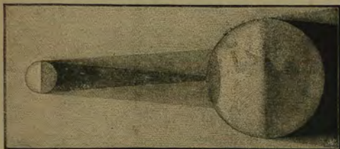
Fig. 66.—Total Eclipse of the Sun; Theory.
