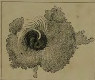
Fig. 19.—Solar cyclone, May 5th, 1857. (Secchi.)
