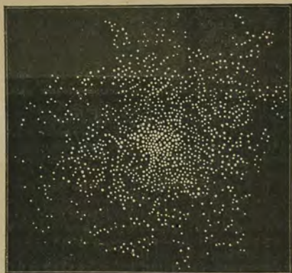
Fig. 148.—Cluster in Aquarius. (Lord Rosse.)
