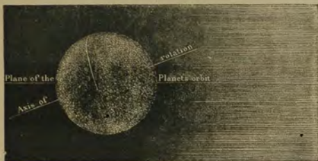
Fig. 37.—Venus at one of its solstices. Inclination of the axis of rotation.
